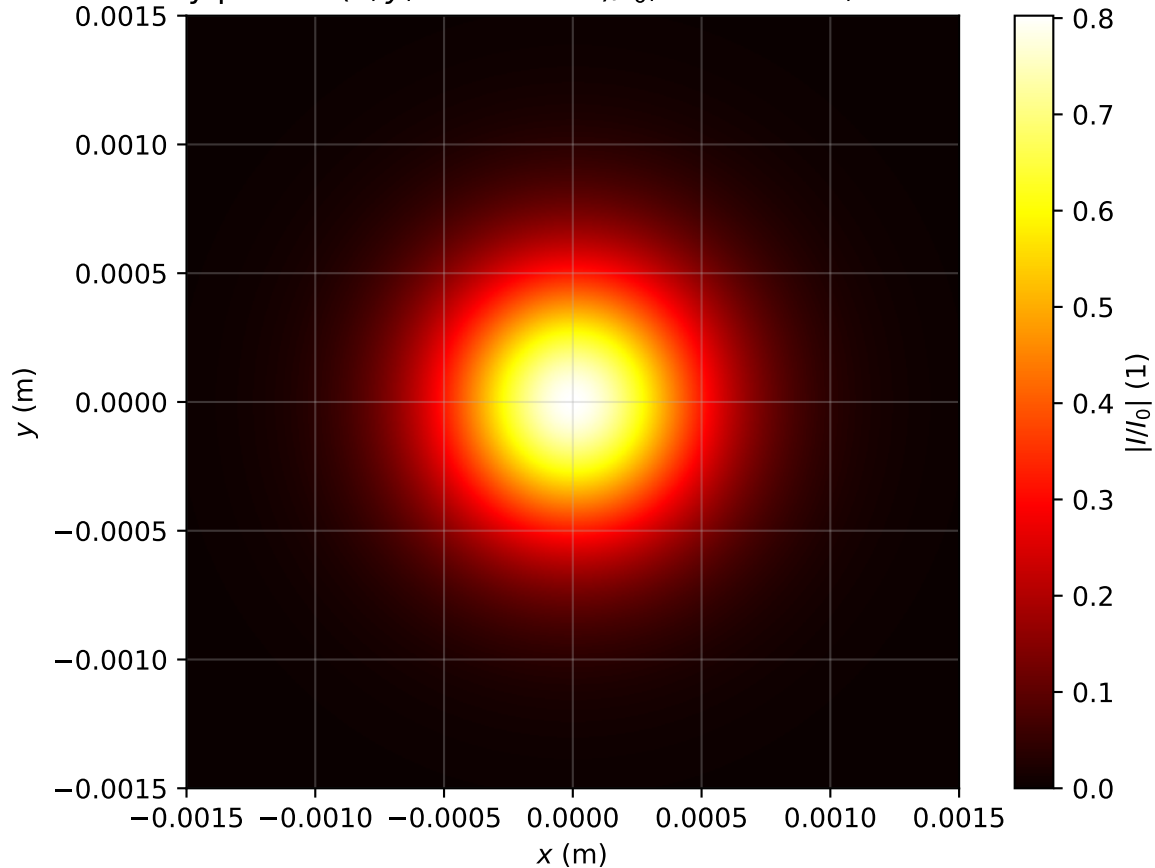
Intensity profile I(x, y, z = 2.070m)/I_0 , Pin=0.5Pcr, artificial time
